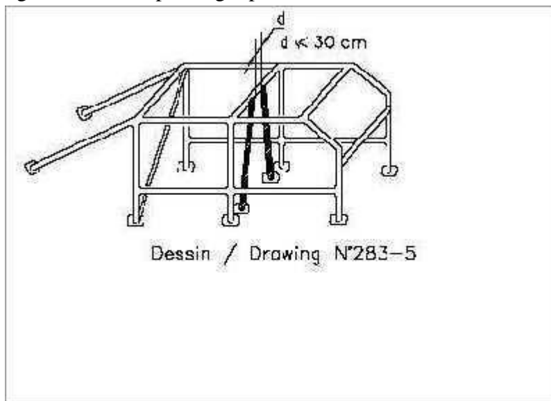
Safety cage TR 2 with 3 passenger place and TR3
